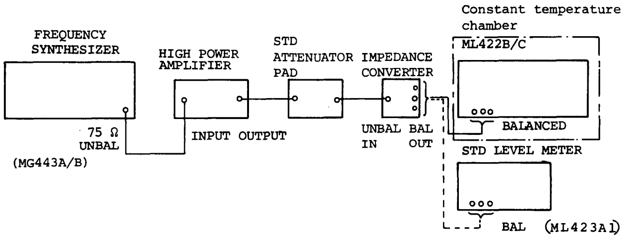
a) Setup for +20 to +10 dBm Measurement
