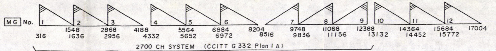
3600 CH SYSTEM (CCITT G 334 Plan 1)
