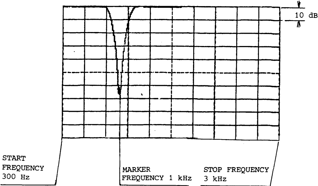
Fig. 4.6 Characteristics of notch filter
