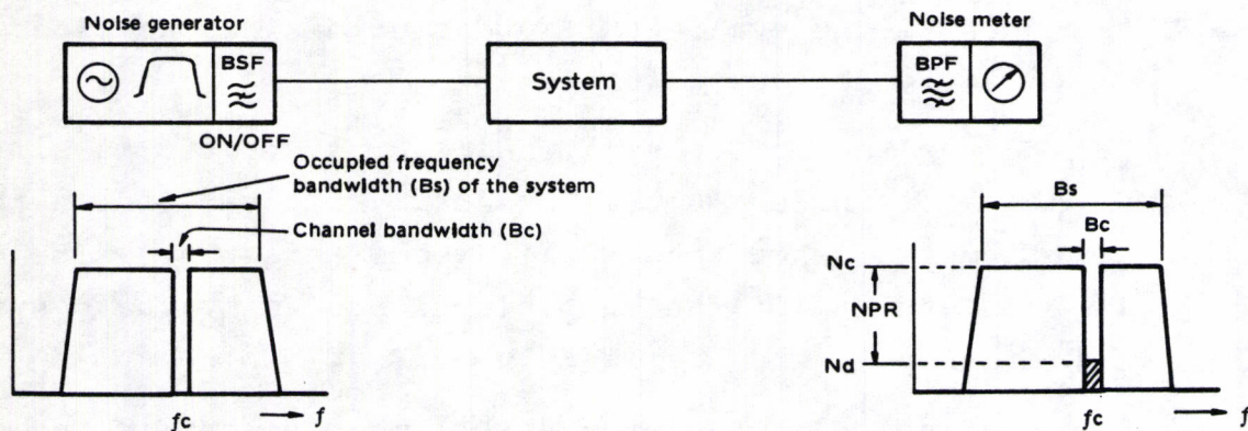
Fig. 2.1-1 NPR Measurement Principle
